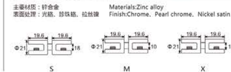
EJ-3058 玻璃夹 Glass holder
