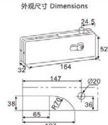
EJ-704 异性夹 Connector patch
