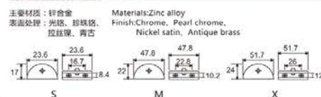
EJ-3052 玻璃夹 Glass holder
