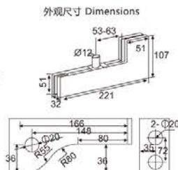
EJ-6040 曲夹 Overpanel corner "L" patch
