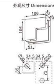
EJ-704 异性夹 Connector patch
