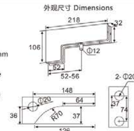
EJ-7040 曲夹 Overpanel corner "L" patch
