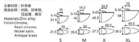
EJ-3051 玻璃夹 Glass holder
