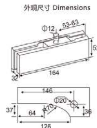
EJ-7030 顶夹 Overpanel pivot patch
