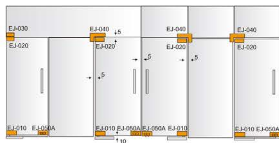
异型门夹扇式样 IRREGULAR PATCH FITTING MODELS
