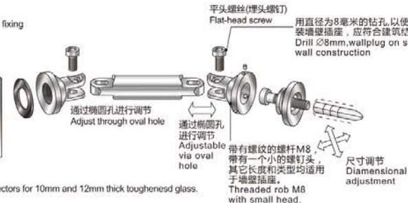
EJ-642 单杆固定件 Ceiling to glass connector CS (墙体与玻璃连接, 单头可调角度) Connection for connecting wall and glass, just one sides can be adjusted angle
