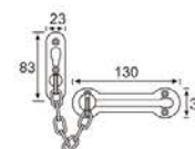
EJ-3043 防盗链 Anti-theft clasp
