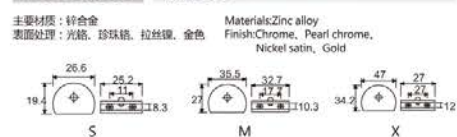
EJ-3053 玻璃夹 Glass holder
