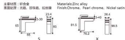
EJ-3050 玻璃夹 Glass holder
