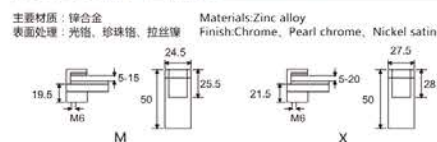
EJ-3049 玻璃夹 Glass holder
