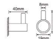
EJ-5035 纸巾架 Tissue Rack
