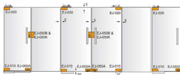
方型门夹扇式样 SQUARE PATCH FITTING MODELS
