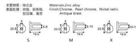
EJ-3057 玻璃夹 Glass holder
