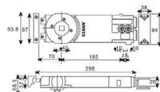
CONCEALED OVERHEAD DOOR CLOSER CENTRE PIVOTED - DOUBLE OR SINGLE ACTING
